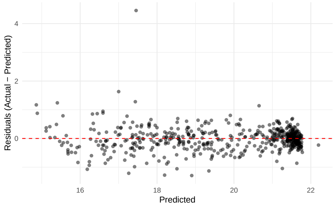
Residuals Plot – Cre
