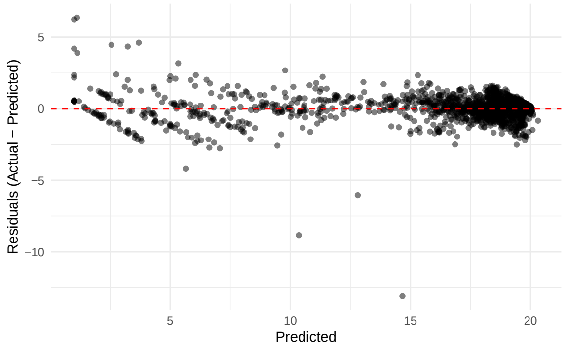
Residuals Plot – SR
