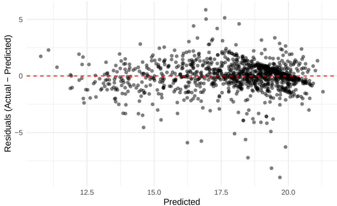
Residuals Plot – TSU
