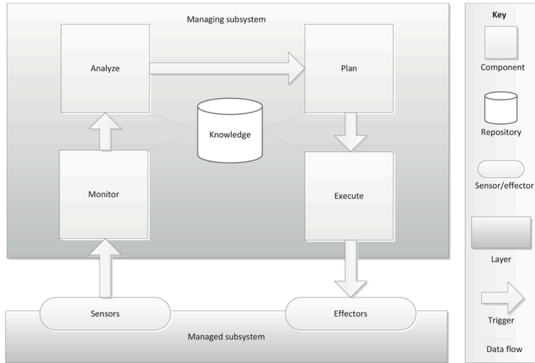
Fig. 1. MAPE-K reference model.
