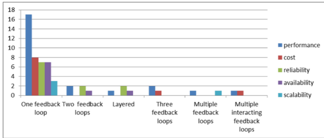
Fig. 9. Feedback loop styles and common QAS.
