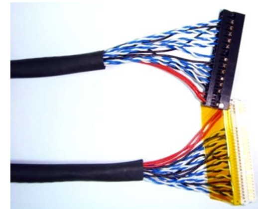
FIX TO 杜邦2.0 UL1571 28AWG
