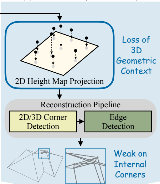
(c) BWFormer (CVPR 2025)
