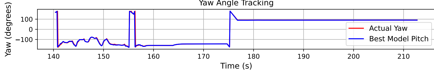
Yaw Angle Tracking
