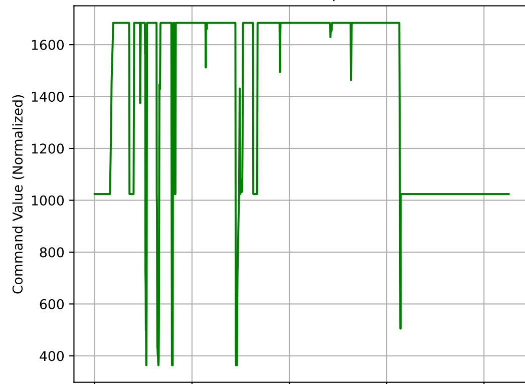
Elevator Input
