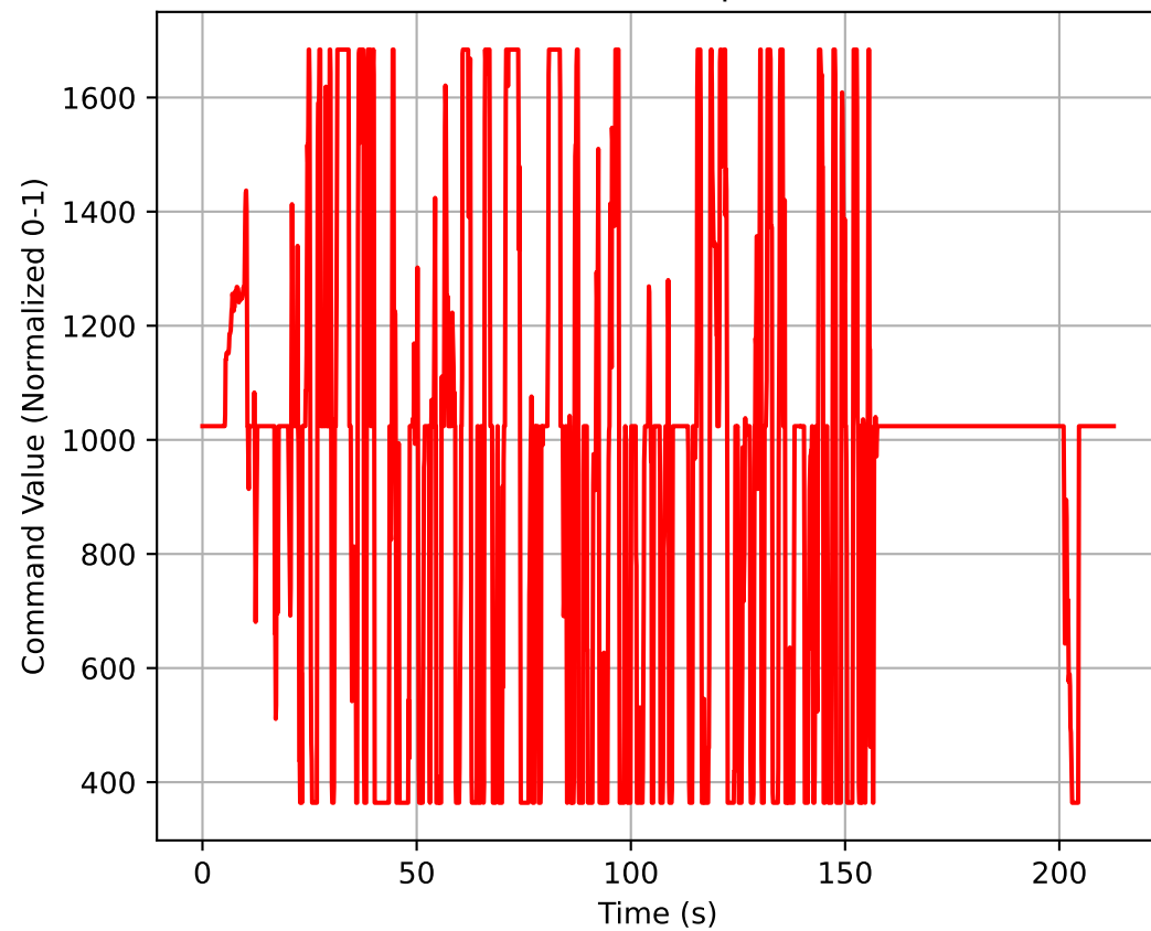
Throttle Input
