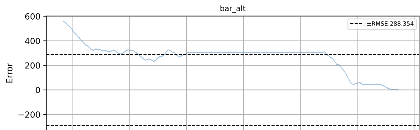
Prediction Errors over Time — Best Model
