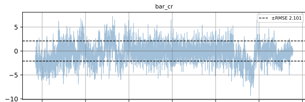
Prediction Errors over Time — Best Model
