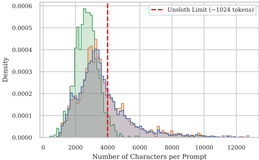
Text Length Distribution (Characters)
