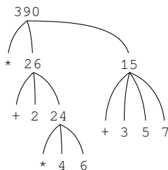
Figure 1.1: Tree representation, showing the value of each sub-combination. 樹表示，展示逐組合值。
