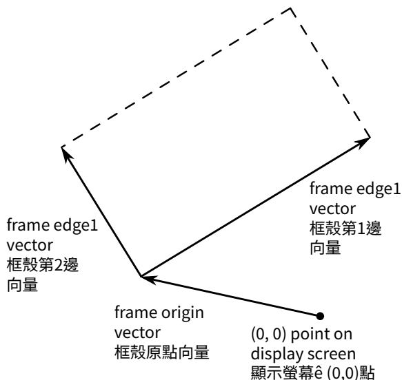
Figure 2.15: A frame is described by three vectors — an origin and two edges. 框殼由三個向量描述——一個原點 \hat{e} 兩個邊 \hat{e} 。
