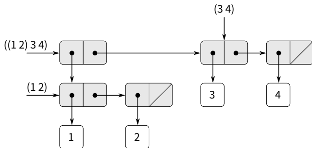
Figure 2.5: Structure formed by (cons (list 1 2) (list 3 4)) . 由 (cons (list 1 2) (list 3 4)) 組成之結構。
