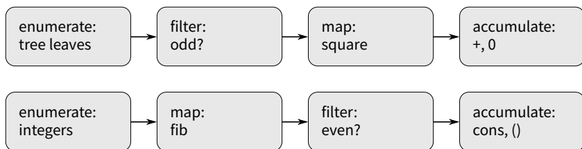
Figure 2.7: The signal-flow plans for the procedures sum-odd-squares (top) and even-fibs (bottom) reveal the commonality between the two programs. 程序 sum-odd-squares (頂 koân ) 和 even-fibs (下底) 的訊號流圖 (signal-flow plans) 顯明兩個程式的共通點。
