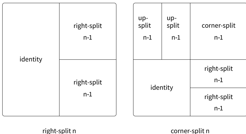
Figure 2.13: Recursive plans for right-split and corner-split. right-split kap corner-split ê 遞迴計畫。
