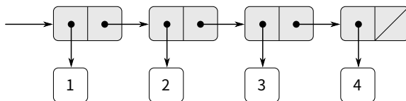
Figure 2.4: The sequence 1, 2, 3, 4 represented as a chain of pairs. 列 1、2、3、4 表達做對的鏈。
