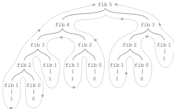
Figure 1.5: The tree-recursive process generated in computing (fib 5). 算 (fib 5) 生成 遞迴過程
