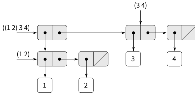
Figure 2.5: Structure formed by (cons (list 1 2) (list 3 4)) .
