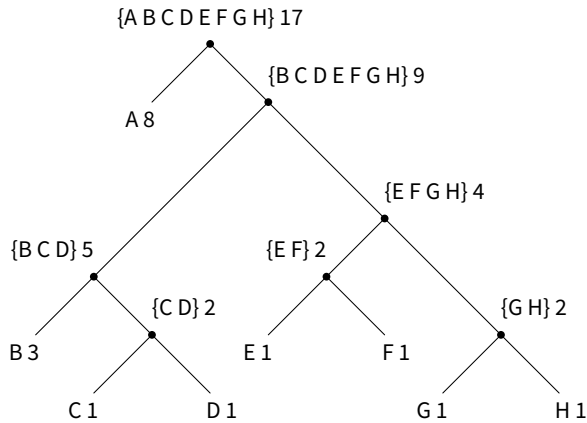
Figure 2.18: A Huffman encoding tree.
