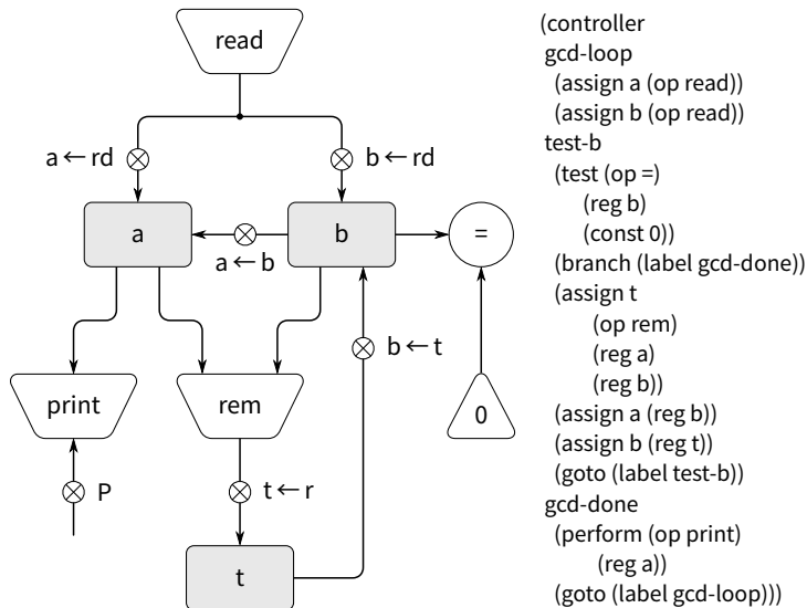
Figure 5.4: A GCD machine that reads inputs and prints results.
