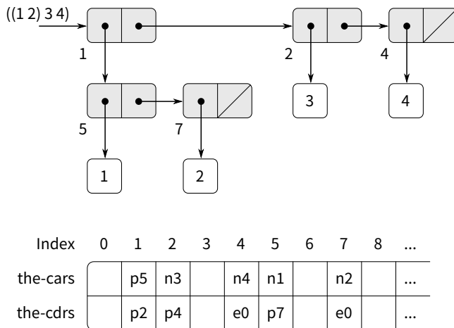
Figure 5.14: Box-and-pointer and memory-vector representations of the list ((1 2) 3 4) .
