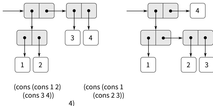
Figure 2.3: Two ways to combine 1, 2, 3, and 4 using pairs.
