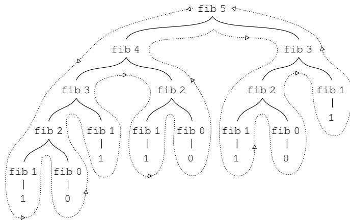
Figure 1.5: The tree-recursive process generated in computing (fib 5). 算 (fib 5) 生成 遞迴樹過程
