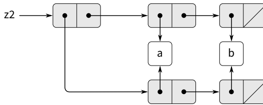
Figure 3.17: The list z2 formed by (cons (list 'a 'b) (list 'a 'b)) .
