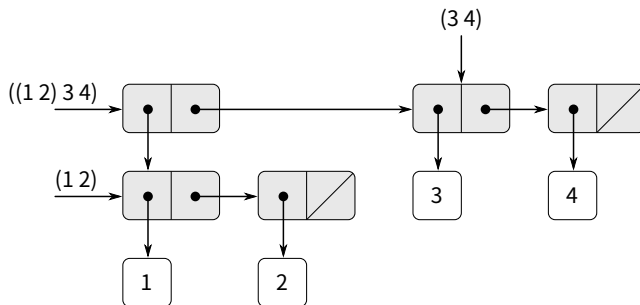
Figure 2.5: Structure formed by (cons (list 1 2) (list 3 4)) .
