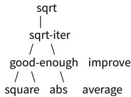
Figure 1.2: Procedural decomposition of the sqrt program.
