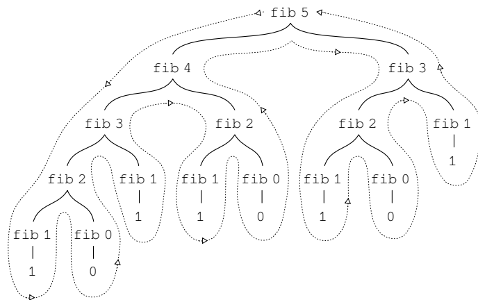
Figure 1.5: The tree-recursive process generated in computing (fib 5).
