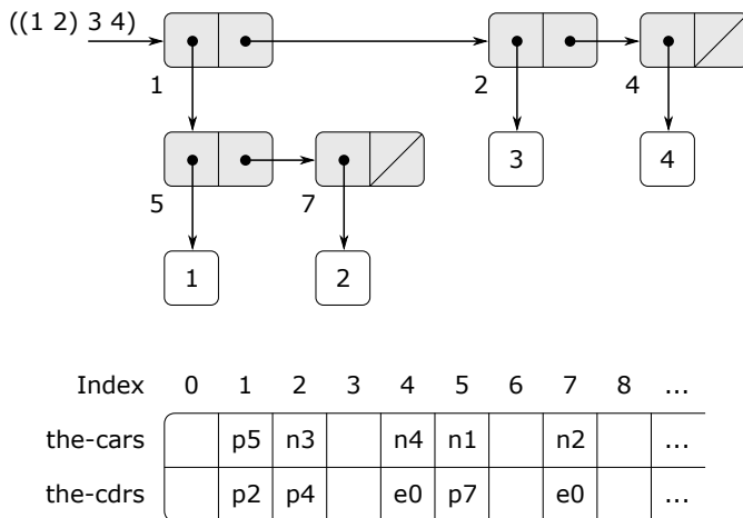
Figure 5.14: Box-and-pointer and memory-vector representations of the list ((1 2) 3 4) .
