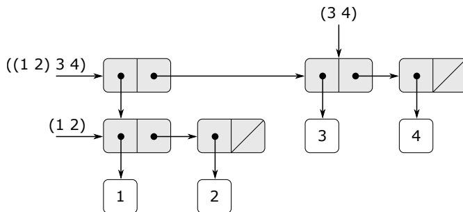
Figure 2.5: Structure formed by (cons (list 1 2) (list 3 4)) .
