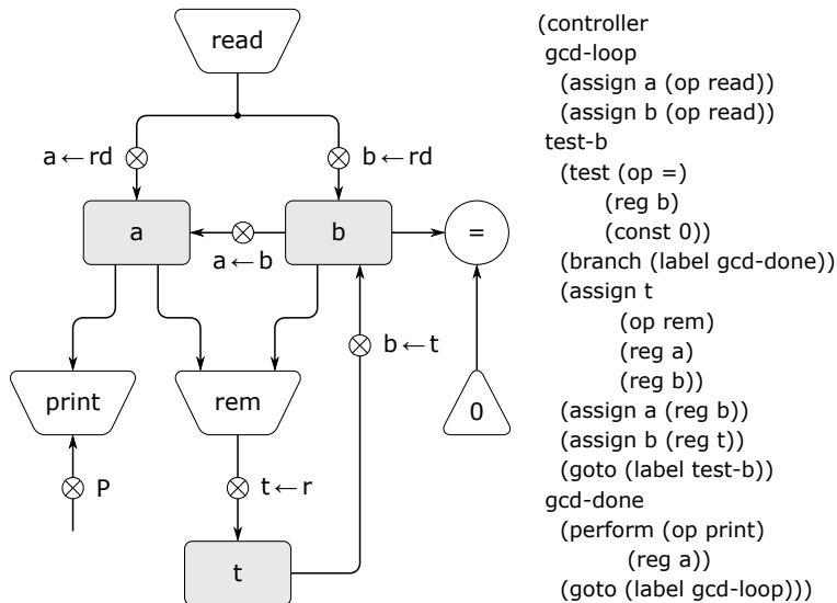
Figure 5.4: A GCD machine that reads inputs and prints results.
