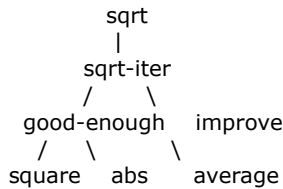
Figure 1.2: Procedural decomposition of the sqrt program.
