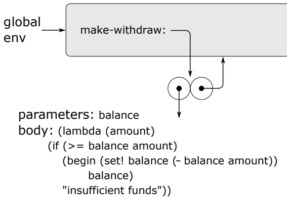
Figure 3.6: Result of defining make-withdraw in the global environment.
