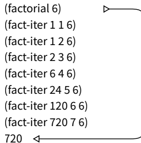
Figure 1.4: A linear iterative process for computing 6! .
