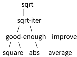
Figure 1.2: Procedural decomposition of the sqrt program.
