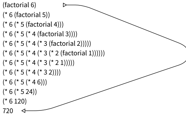
Figure 1.3: A linear recursive process for computing 6! .
