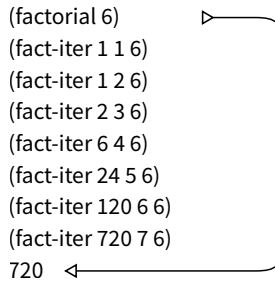
Figure 1.4: A linear iterative process for computing 6! .
