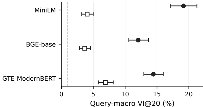
(a) Visibility instability
