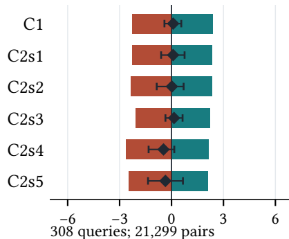
WANDS / BGE / K = 20
