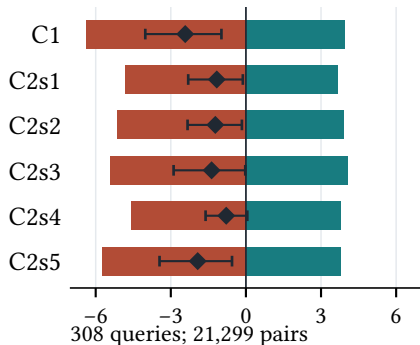
WANDS / MiniLM / K = 100
