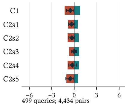
ESCI / BGE / K = 20
