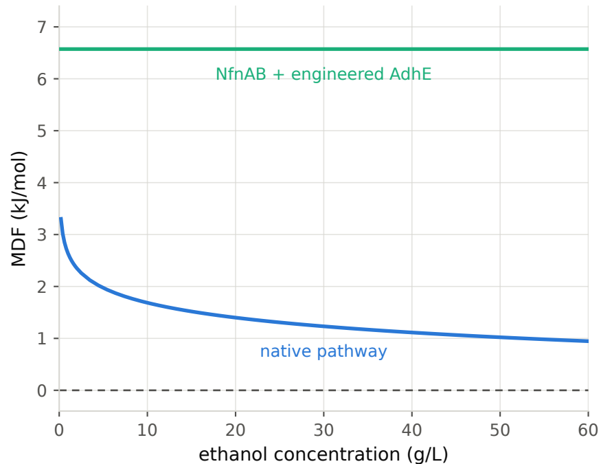
Driving force lost to product accumulation
