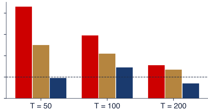
GARCH(1,1) errors
