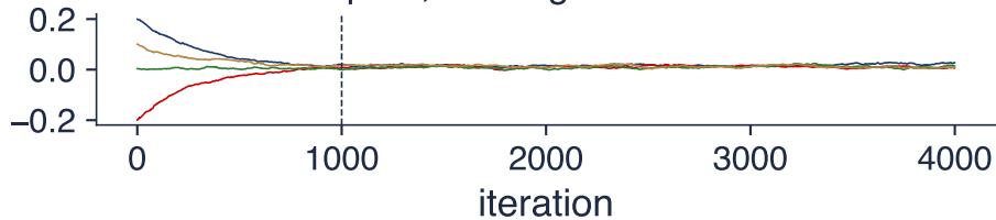
Slope b, raw regressor: traces
