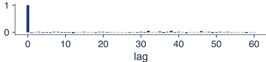
Slope b, centred regressor: autocorrelation of the draws
