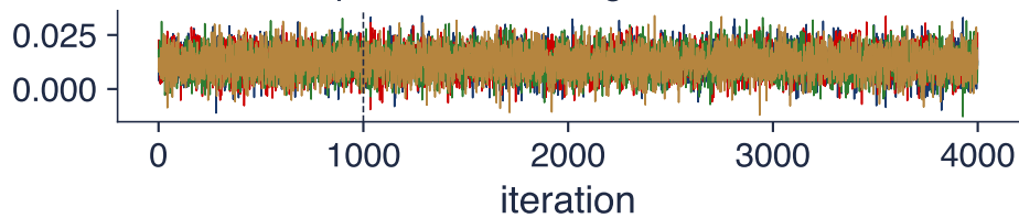
Slope b, centred regressor: traces
