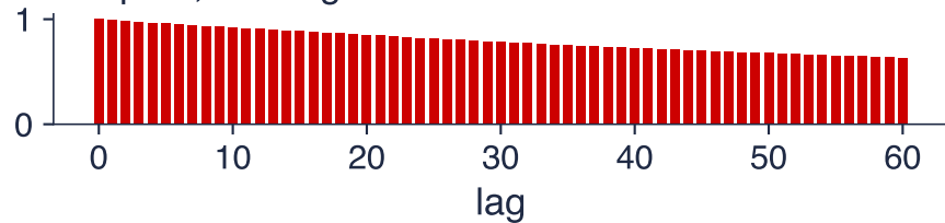
Slope b, raw regressor: autocorrelation of the draws
