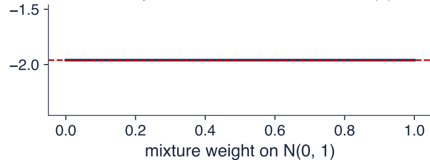
Same quantile: Normal and rescaled t(3)
