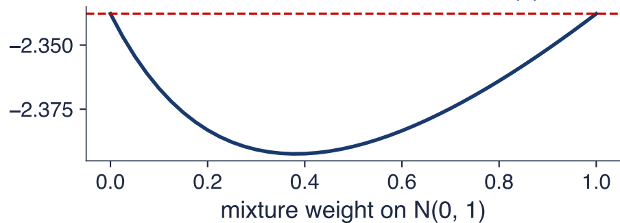
Same ES: Normal and rescaled t(3)
