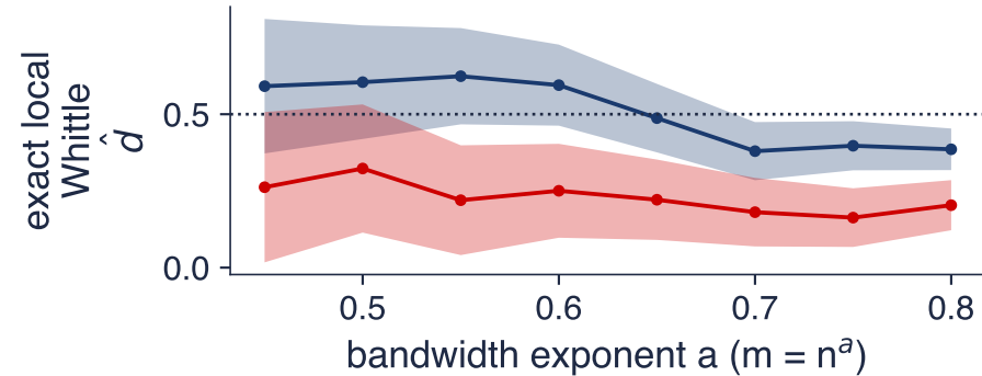
United States, CPI
