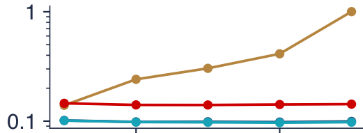
DGP: MA(1)
