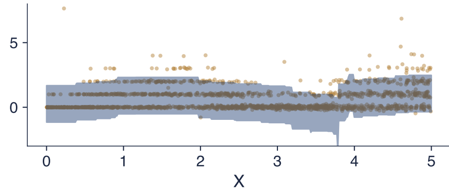
split conformal (mean model)
