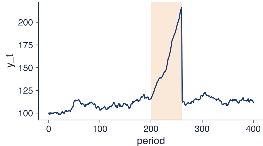
Bubble-and-collapse process, T = 400
