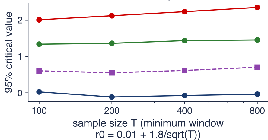
Critical values against T
