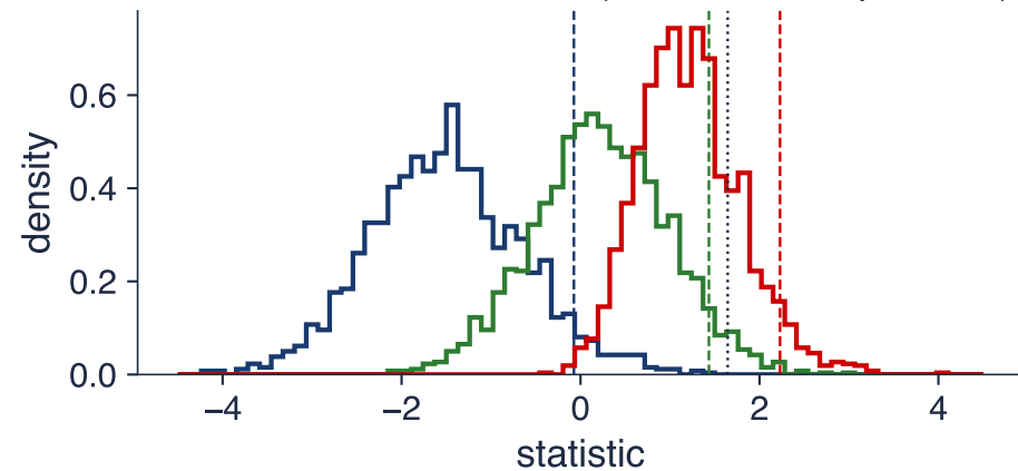
Null distributions, T = 400 (dashed: 95% quantiles)
