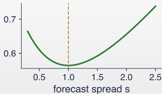
— expected CRPS - - - true spread s = 1
