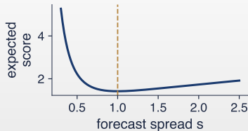
— expected log score - - - true spread s = 1
