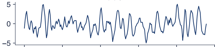
AR(2) path
