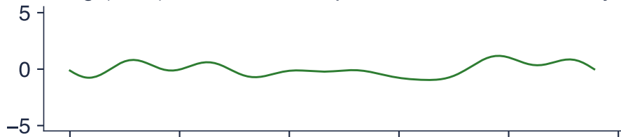
long ( > 32 ): 8% of the sample variance, 9% in theory
