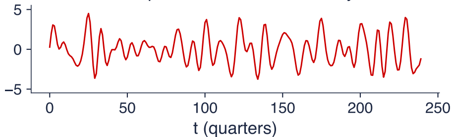
business cycle (6-32): 84% of the sample variance, 84% in theory
