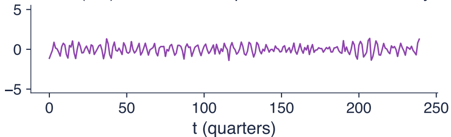
short ( < 6 ): 8% of the sample variance, 7% in theory
