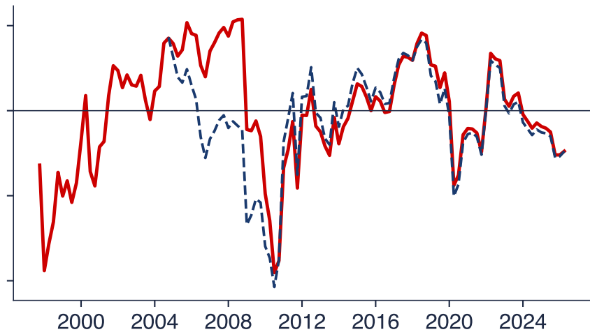
Hamilton filter, h = 8 , p = 4
