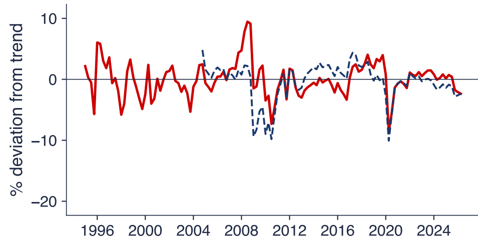
HP filter, \lambda = 1600
