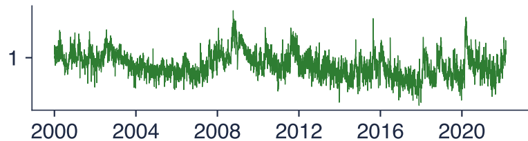
— S&P 500 realised variance ( \%^2 )
