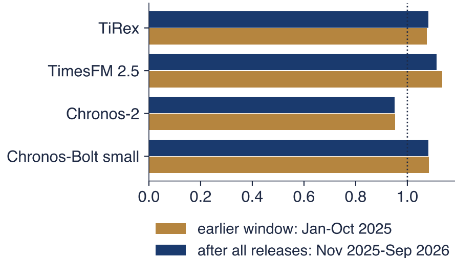
Romanian load: MAE / expert ARX
