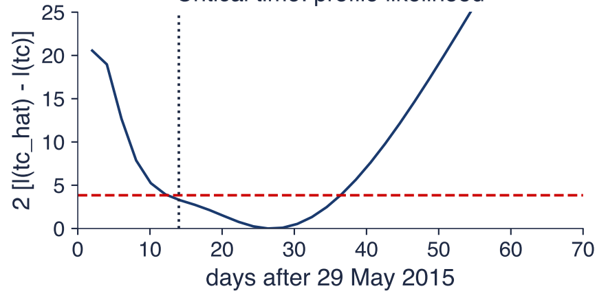
Critical time: profile likelihood
