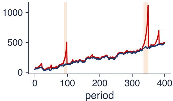
Evans (1991) bubble
