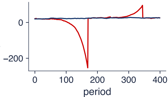
Blanchard-Watson bubble
