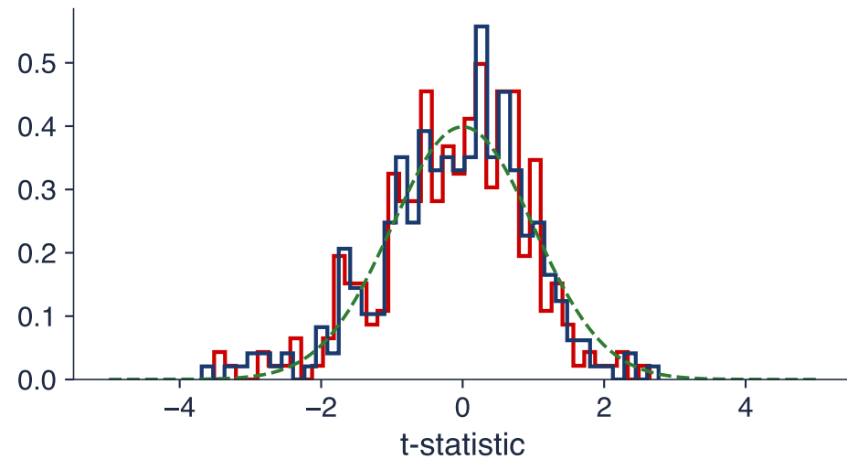
Gaussian innovations
