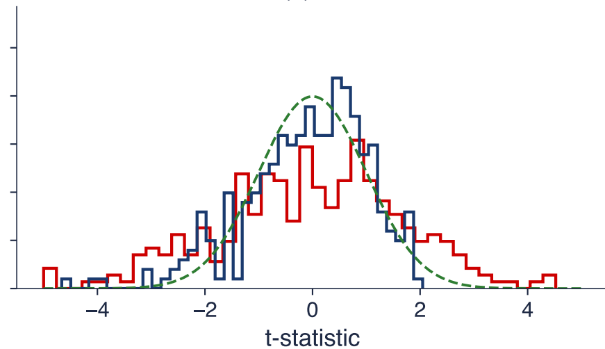
Student-t(5) innovations
