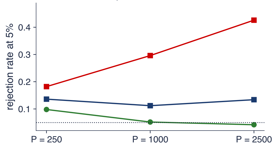
Kupiec test, VaR 1%
