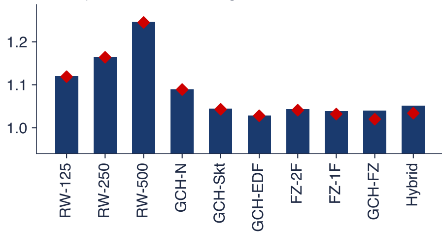
alpha = 0.025: average FZ0 loss, 2000-2016
