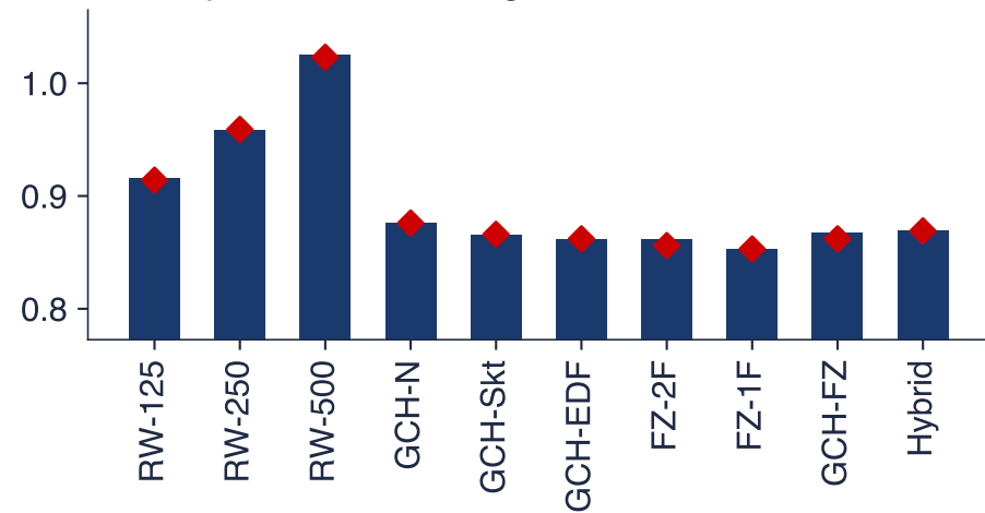
alpha = 0.05: average FZ0 loss, 2000-2016
