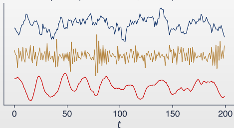
Simulated paths (standardised, shifted)
