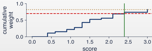
— cumulative weight ⋯ 1 - \tilde{w}_{n+1} --- 1 - \alpha = 0.7 | weighted \hat{q}
