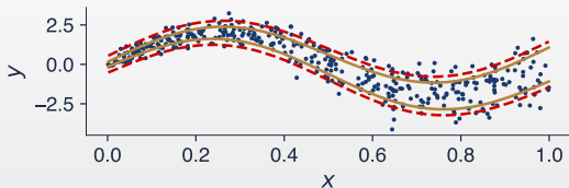
• test points --- CQR band, \pm \hat{q} — raw 10%, 90% quantiles
