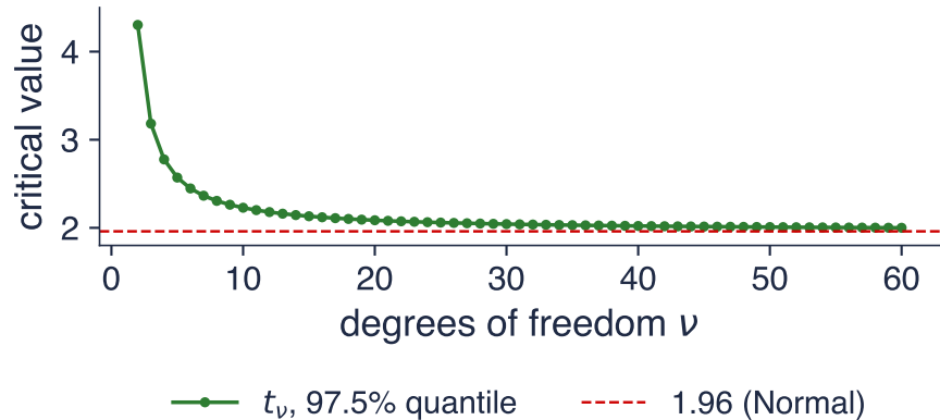
EWC: Student- t_\nu , two-sided 5%
