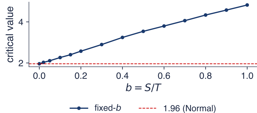
Bartlett kernel, two-sided 5%
