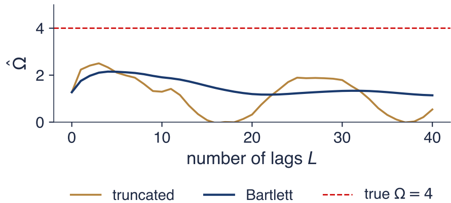
\hat{\Omega} , one AR(1) sample, \phi = 0.5
