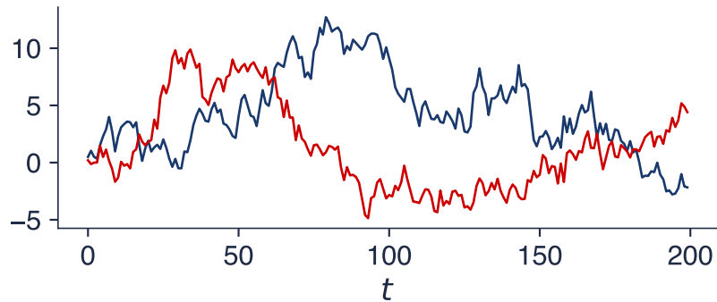
Two independent random walks
