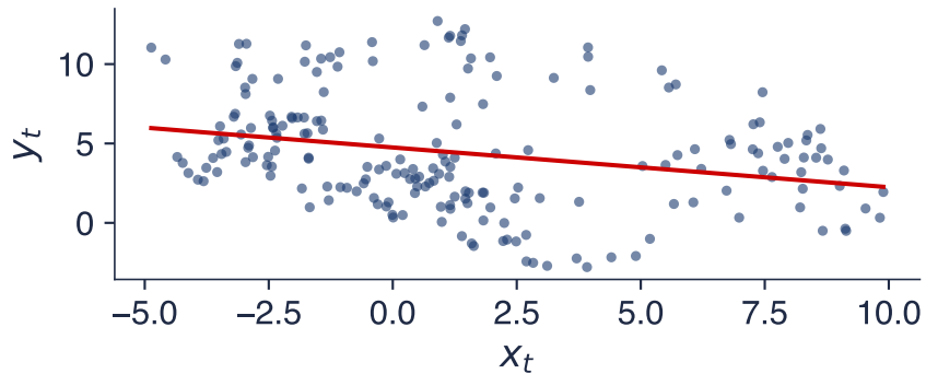
Regression of y_t on x_t
