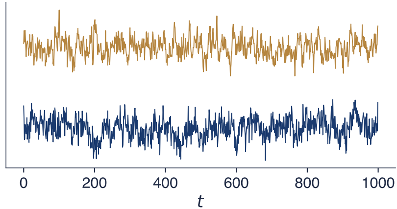
Simulated paths (same variance, shifted)
