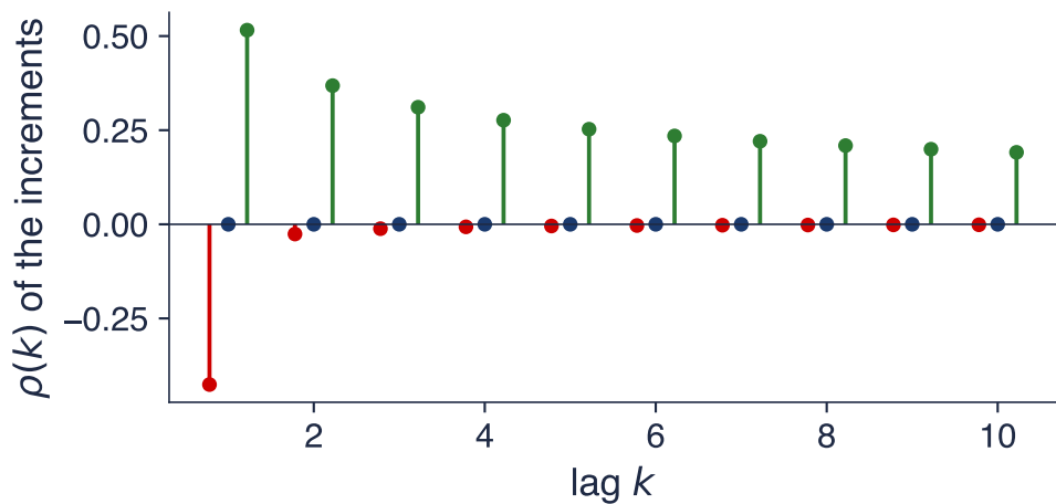
Fractional Gaussian noise
