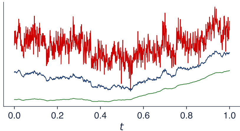
Paths of W_t^H (shifted vertically)
