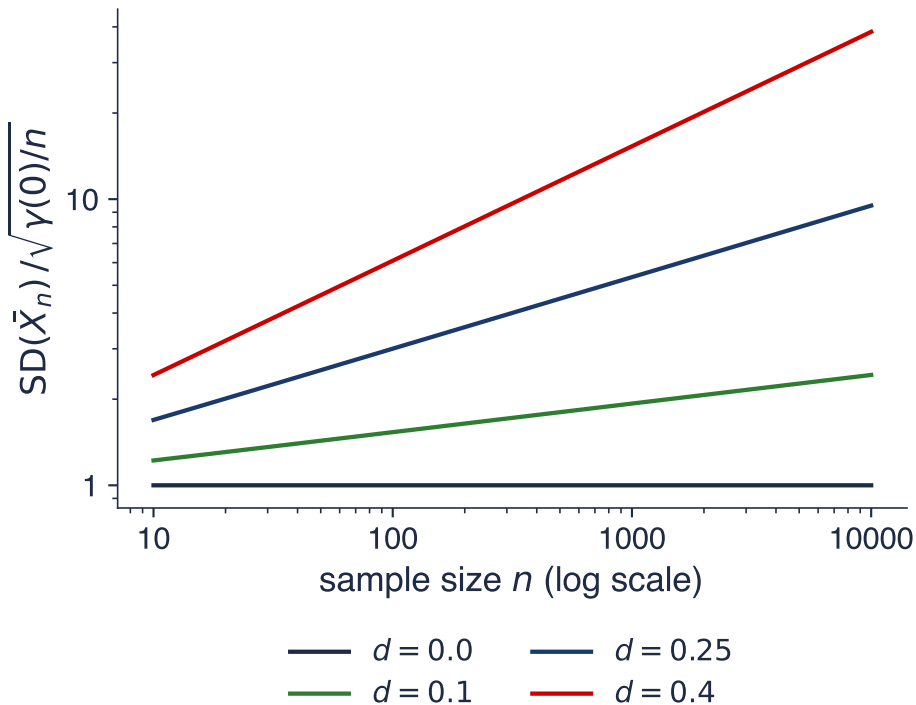
True SD of the mean over the i.i.d. formula
