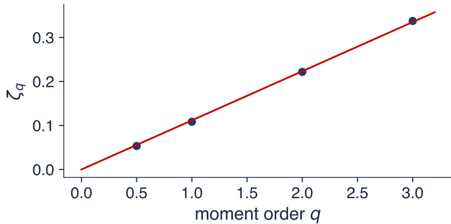
Simulated rough log volatility, H = 0.12
