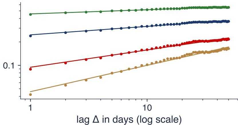
Moments of |\log \sigma_{t+\Delta} - \log \sigma_t|^q
