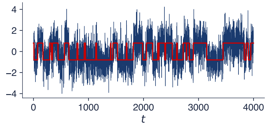
Markov switching: stay probability q = 0.99
