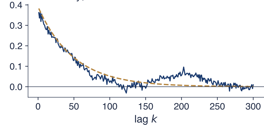
Slow decay; local Whittle \hat{d} = 0.52
